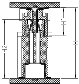
Assembly
