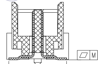
SECTION E-E SCALE 2:1
